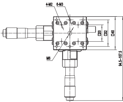
NFP-3461CCZ-L
